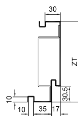
V-UD-30 / LBW Plan T3162
