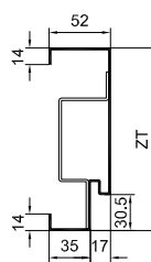
W-UD-30 / LBW Plan T3161
