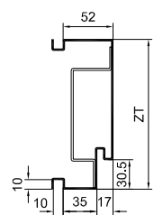
WV-UD-30 / LBW Plan T3163
